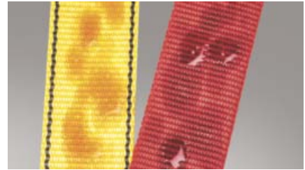
Harness without NanoSphere coating absorbs oil and water
