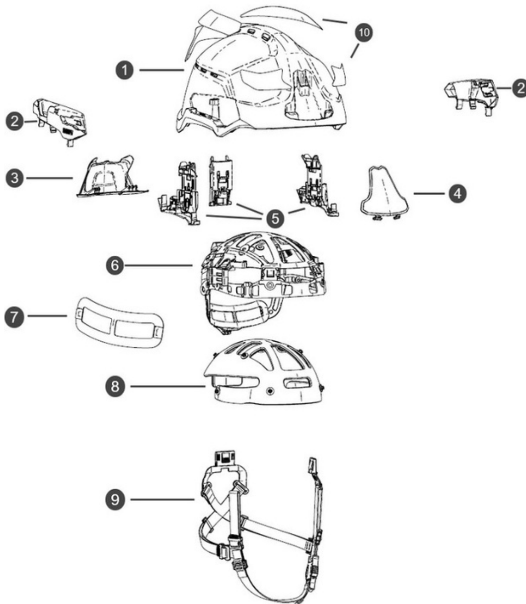
Figure 2 Exploded View
